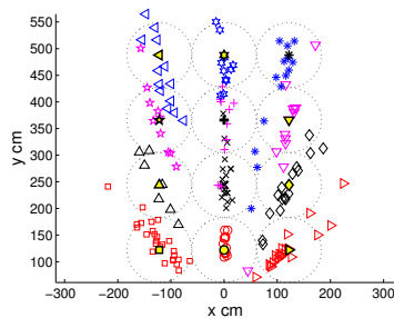
Fig. 13: Field test localization map. The dotted circle has a reference radius as 61cm. Each listener is located at the center of each circle. Results are denoted using same maker as the target’s ground truth location.
