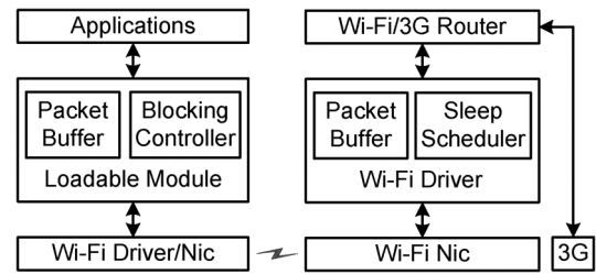
Fig. 10. Implementation architecture of (left) the client part and (right) the softAP part.
